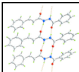
Fig. 2. Supramolecular tape with undulating topology in (I). The N-H \cdots O hydrogen bonding is shown as orange dashed lines
